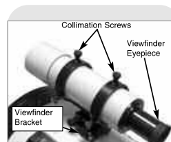
Fig. 14a: Viewfinder assembly, refractor and Schmidt-Newtonian mod-
