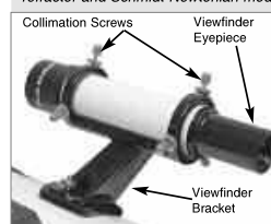
Fig. 14b: Viewfinder assembly, Newtonian models.
