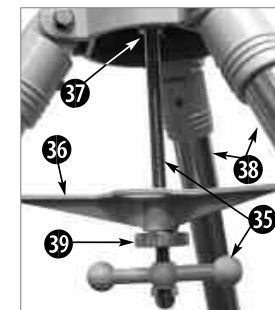
Fig. 1c: The LX D75-Series Tripod.
