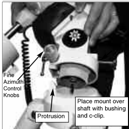
Fig. 5c: Attach the mount to the tripod.
