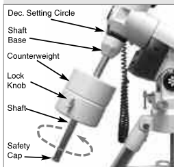
Fig. 6: Attach counterweight assembly.
