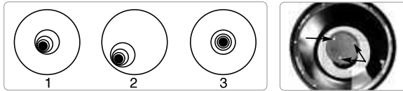
Fig. 33a: Defocused star images. Misaligned (1, 2), Aligned (3)
