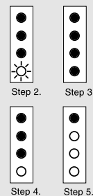
Fig. 52a: Indicator Light Key for changing tracking rates in the Northern Hemisphere Polar mode.
