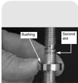
Fig. 5a: Slide bushing over shaft.
