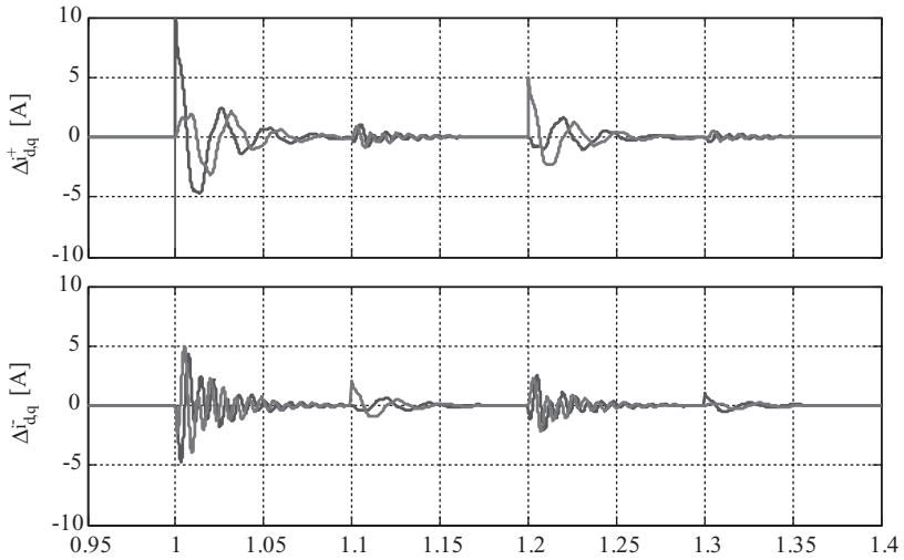
Figure 10.7 Error signals on the double synchronous reference frame controller using notch filters on the measured currents ( d error current signal in black and q error current signal in gray)
