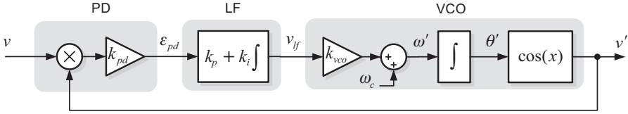
Figure 4.5 Block diagram of an elementary PLL
