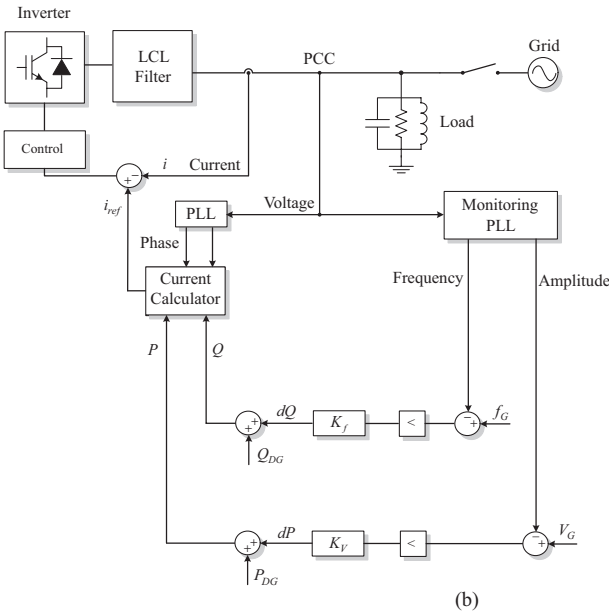
Figure 5.7 (a) Frequency and voltage positive feedback flowchart and (b) control scheme.
