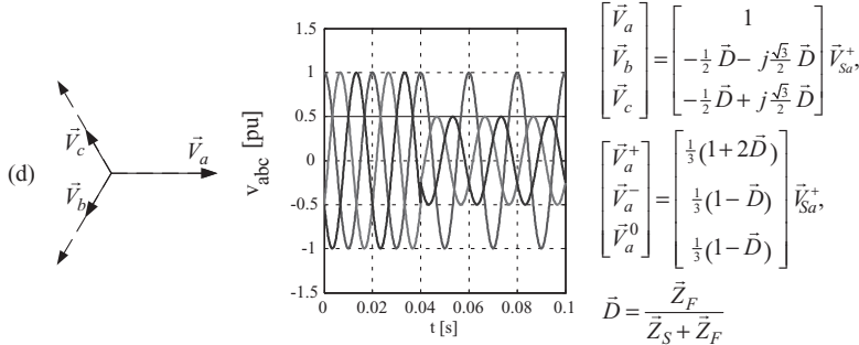
Figure 8.6 Voltage sags due to grid faults in three-phase systems with \vec{D} = 0.5\angle 0^\circ
