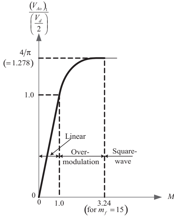
Figure 12.24 Range of linear operation
