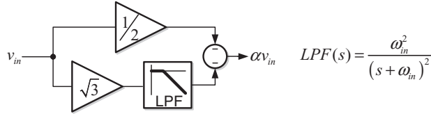
Figure A.3 Simple implementation of the a operator in the time domain
