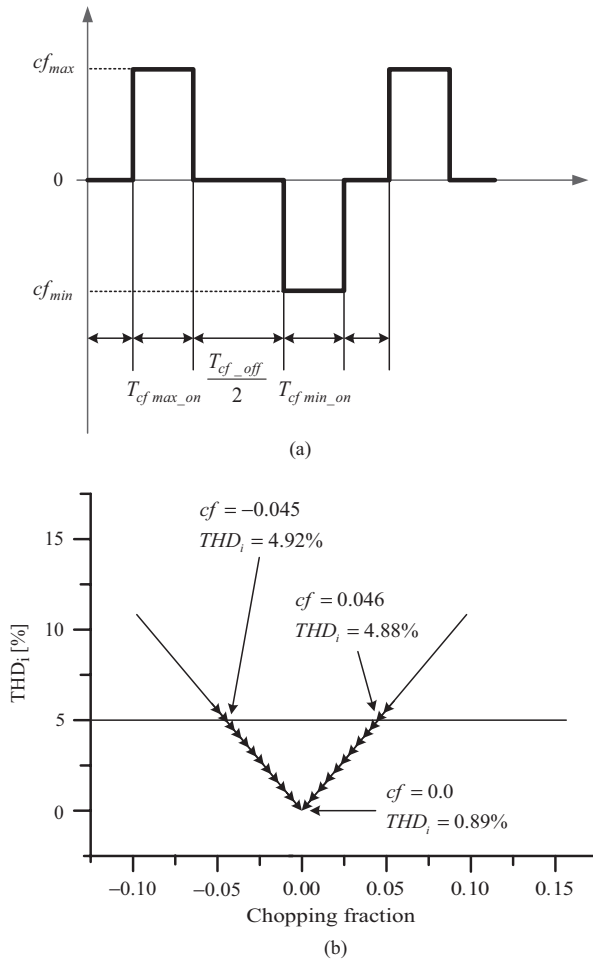
Figure 5.6 (a) Chopping fraction in AFDPCF and (b) current THD_i as a function of the chopping fraction
