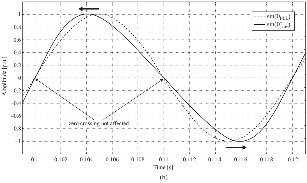
Figure 5.13 (a) The effect of the injected signal ( \sigma_{inj} ) for the grid current reference in p.u. ( \sin(\theta_{inv}^*) ) at normal operation and (b) when the amplitude of the injected signal is 10 times larger than necessary in order to illustrate the method
