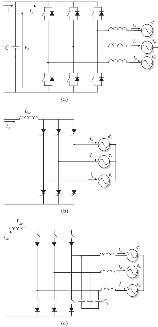
Figure 6.6 Grid converter in the case of indirect type conversion: (a) forced-commutated VSI, (b) phase-controlled line-commutated converter and (c) forced-commutated CSI
