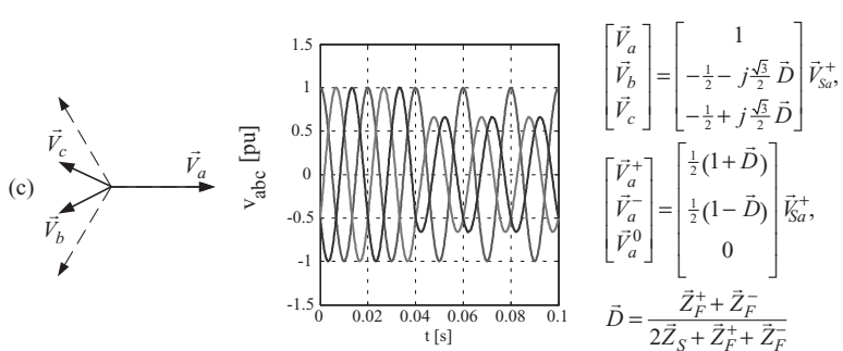
Sag type E. Two-phase to ground fault
