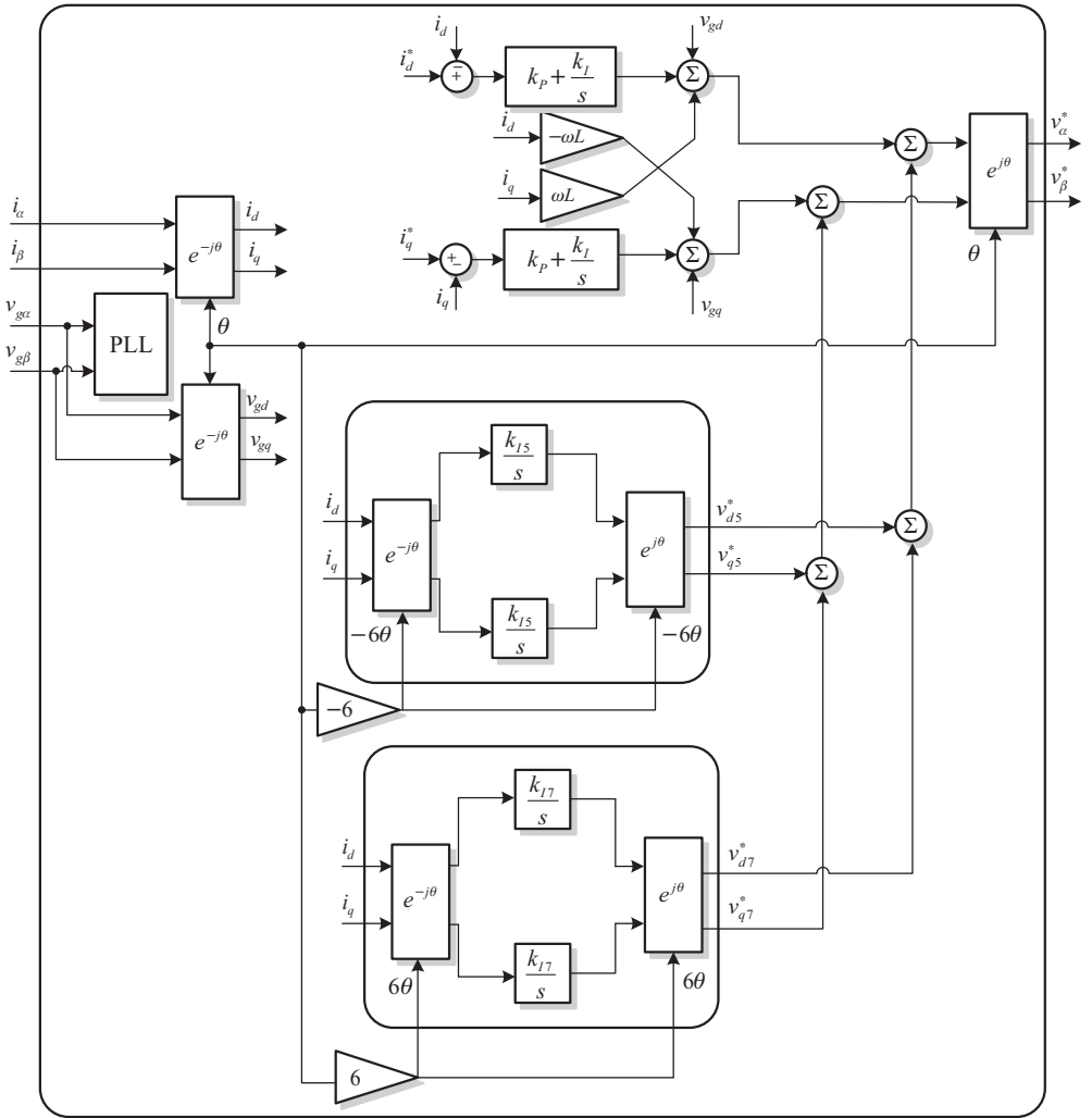
Figure 12.21 Current control structure of the three-phase grid inverter with 5th and 7th harmonic compensation using 6th and -6\theta dq reference frames nested in the main
