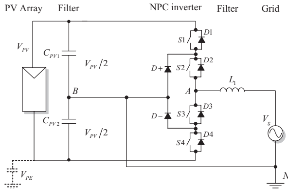
Figure 2.15 Neutral clamped half-bridge
