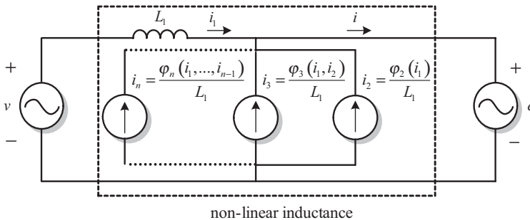
Figure 11.23 Volterra-based model of the nonlinear inductance connected between the inverter v and the grid e
