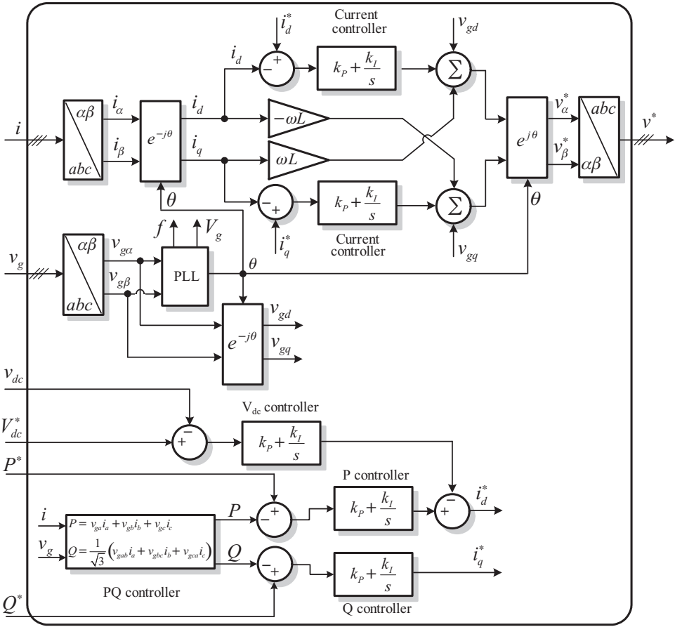
Figure 12.7 Synchronous PI dq current control for three-phase voltage-source grid converters
