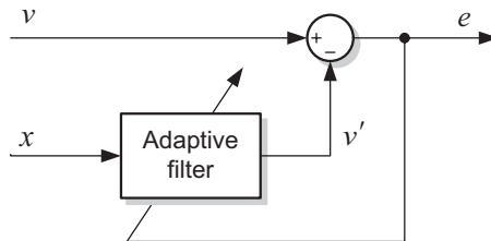
Figure 4.19 Adaptive noise cancelling (ANC) system
