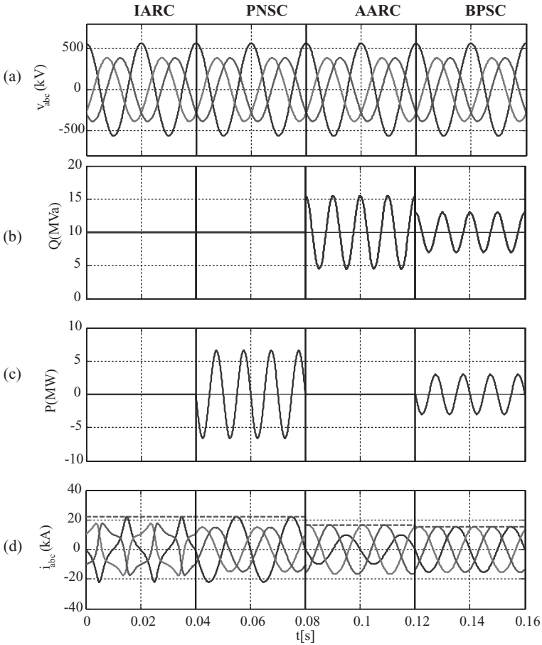
Figure 10.16 Simulation of the IARC ( t = 0 to t = 40 ms), PNSC ( t = 40 ms to t = 80 ms), AARC ( t = 80 ms to t = 120 ms) and BPSC ( t = 120 ms to t = 160 ms): (a) unbalanced voltage measurement, (b) injected reactive power, (c) delivered active power and (d) injected currents
