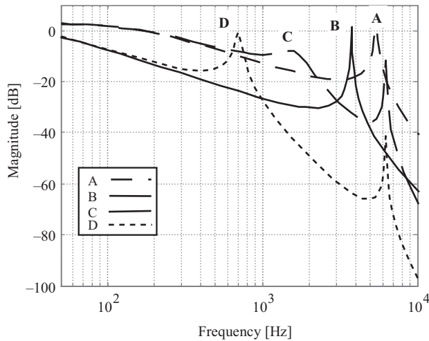
Figure 11.8 Frequency characteristic of the 3 kW PV system with an LCL filter in the following grid conditions: A: 0.1 mH, B: 3 mH, C: 0.1 mH, 100 \mu\text{F} , D: 3 mH, 100 \mu\text{F}
