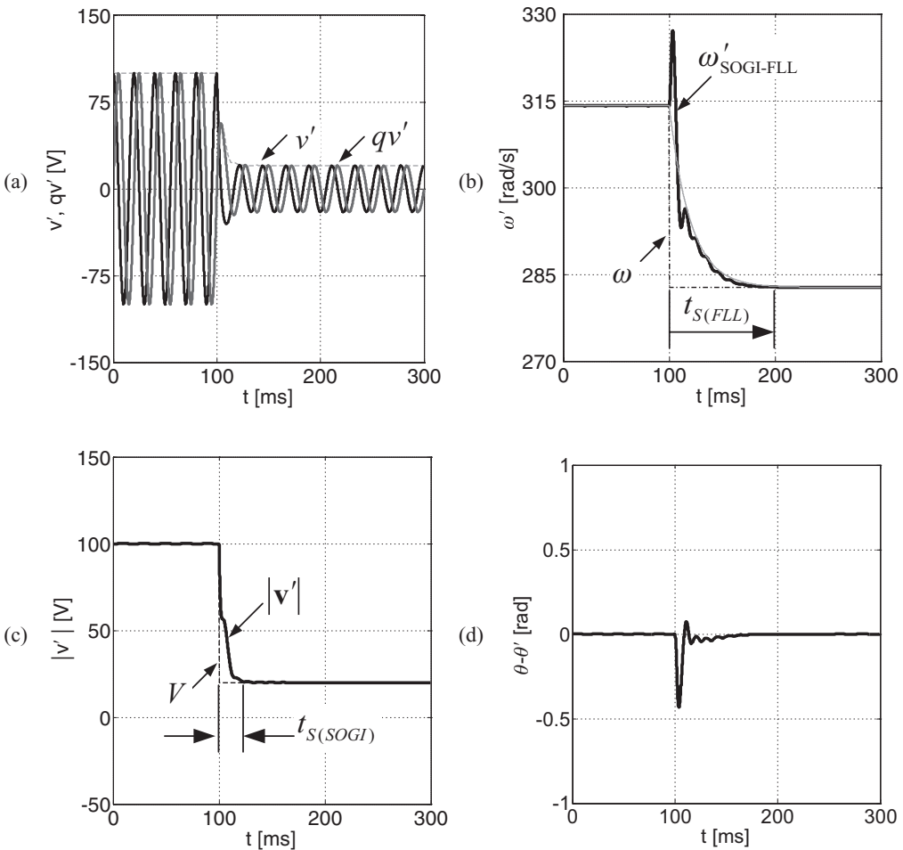
Figure 4.36 Response of the SOGI-FLL with FLL gain normalization when the input signal simultaneously experiences a voltage dip and a frequency jump: (a) in-quadrature signals, (b) detected frequency, (c) detected input voltage amplitude and (d) error in phase-angle detection \theta - \theta'
