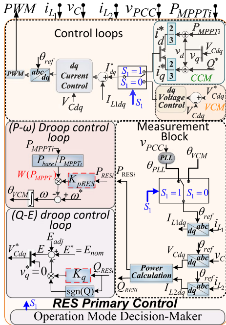
Fig. 13. Scheme of the primary control for RESs.
