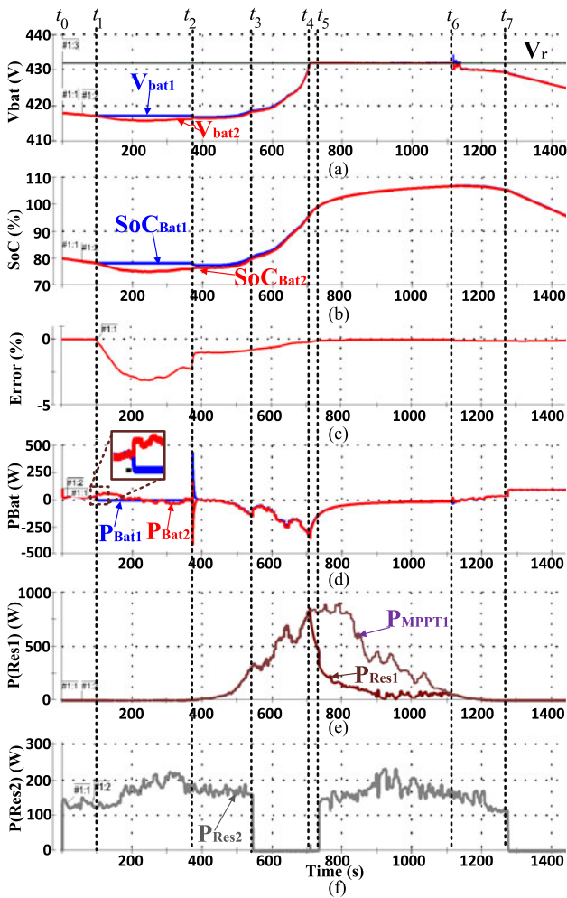
Fig. 22. Experimental performance for one day of operation.
