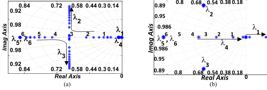
Fig. 14. Root locus plot for TCM1 and TCM3 varying: (a) K_p ; (b) K_q .
