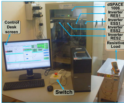
Fig. 18. Experimental setup at the laboratory.
