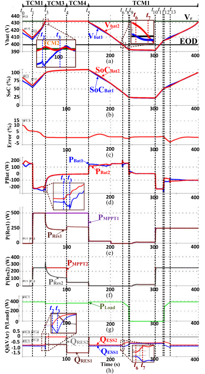
Fig. 19. Experimental results for all TCM.
