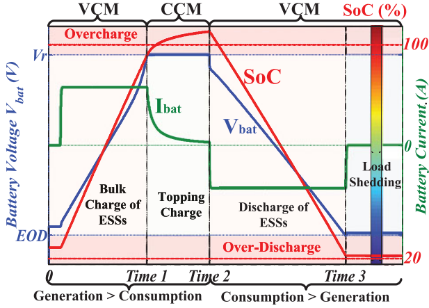
Fig. 2. Charging profile for lead-acid batteries.
