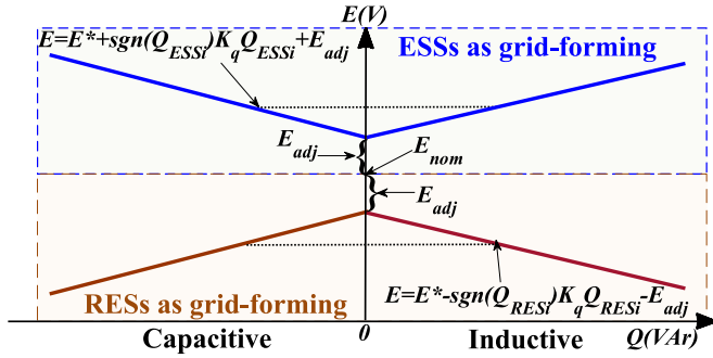
Fig. 7. Proposed (Q - E) droop characteristics.
