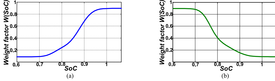
Fig. 11. Control curves of the FIS: (a) Charge; (b) discharge.
