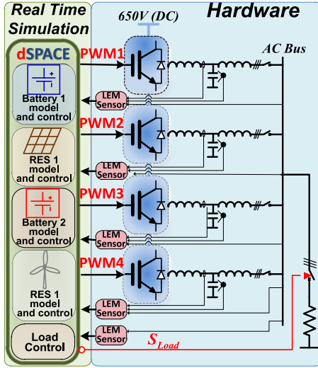
Fig. 17. Scheme of the experimental setup.
