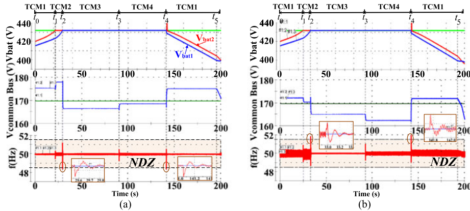
Fig. 21. Voltage/frequency signaling: (a) capacitive load; (b) inductive load.
