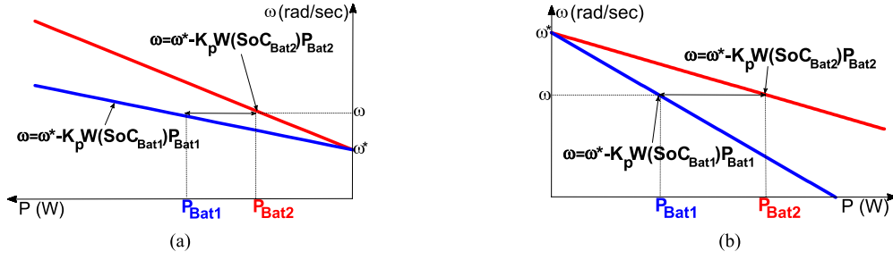
Fig. 10. Active power sharing with weighted droop coefficients for (a) ESSs charge and (b) ESSs discharge.
