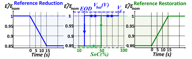
Fig. 8. Adaptive voltage pattern for LS.
