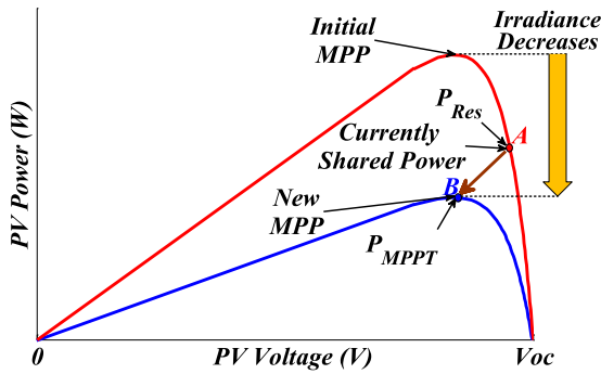
Fig. 5. Effect in the power generation from RESs when a RES initially working in VCM reduces its maximum power below the current shared power ( P_{MPPTi} < P_{Resi} ), (Ev 2 ).
