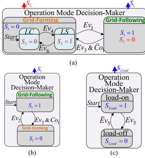
Fig. 9. DM units based on FSM for (a) ESSs, (b) RESs, and (c) loads.
