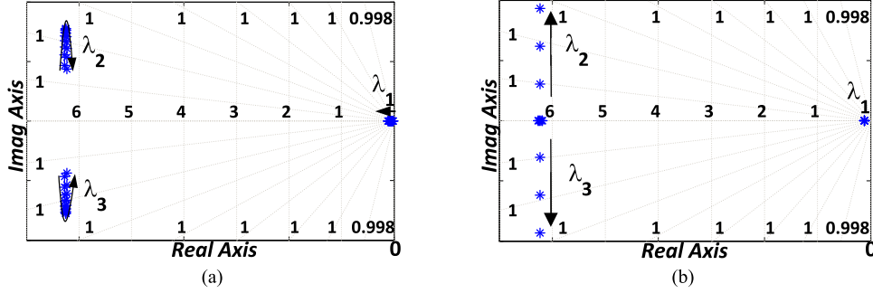
Fig. 15. Root locus plot for TCM2 and TCM4 varying: (a) K_p ; (b) K_q .
