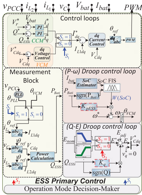
Fig. 12. Scheme of the primary control for ESSs.
