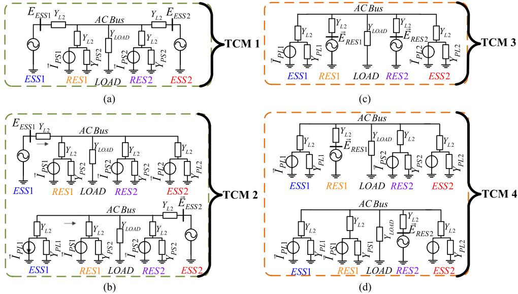
Fig. 4. TCM for islanded microgrid.
