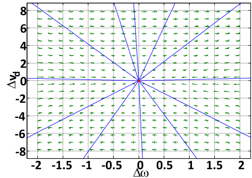
Fig. 16. Phase portrait for the linear approximation system in (14).
