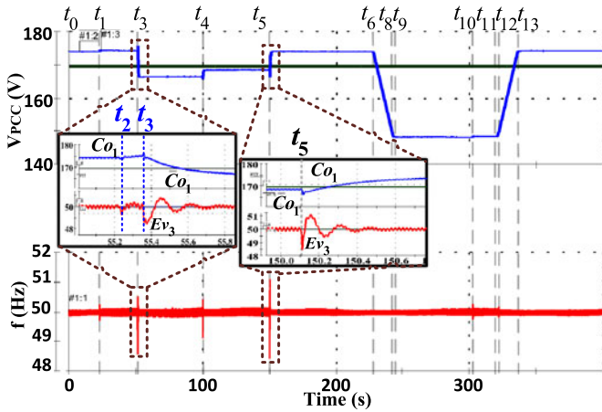
Fig. 20. Common bus voltage and frequency.
